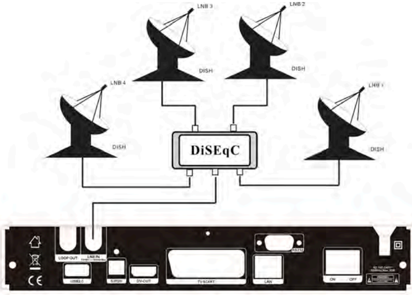
Figure7. Connecting to Dish LNB
