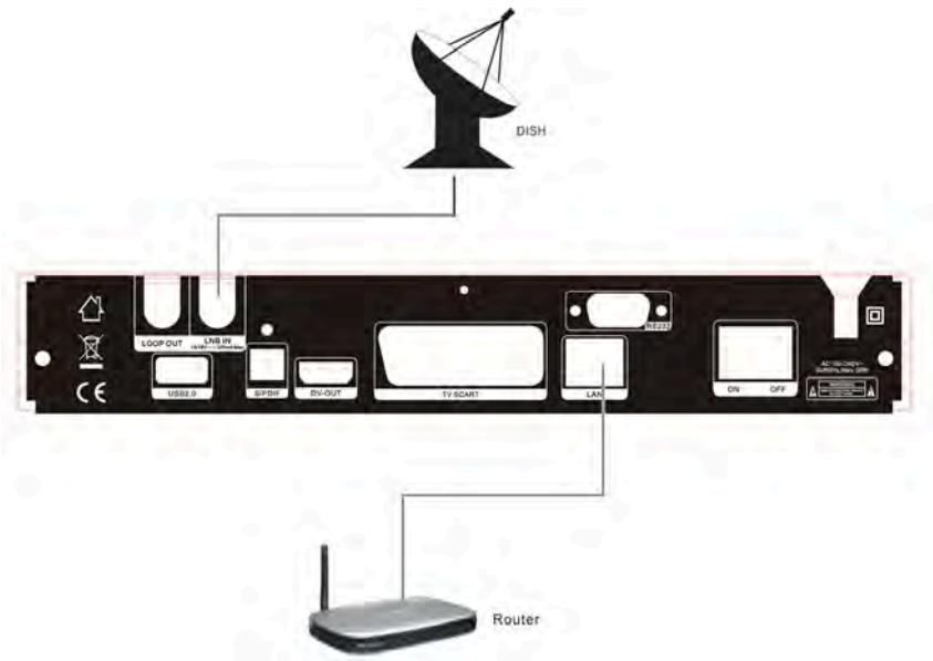
Figure6. Connecting to Dish LNB
